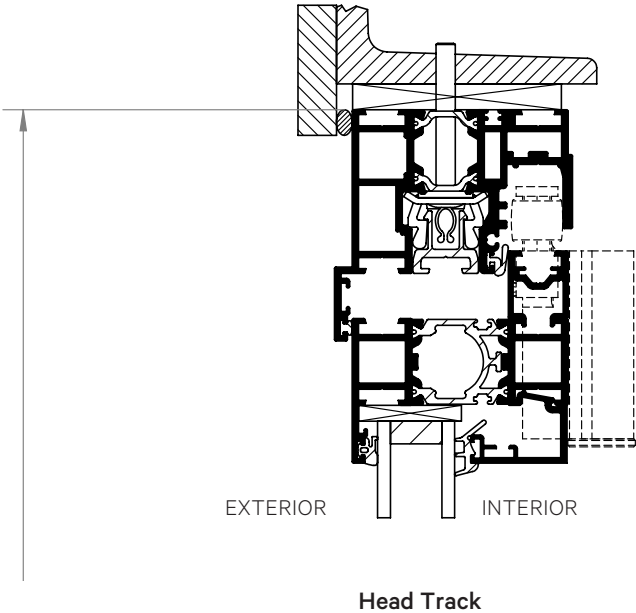
Head Track
